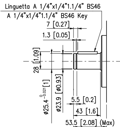
ALBERO SHAFT C25.4
