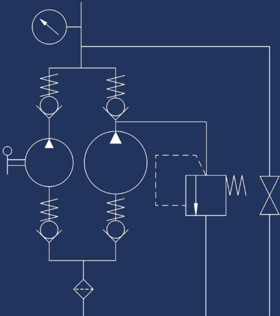
HYDRAULIC DIAGRAM
