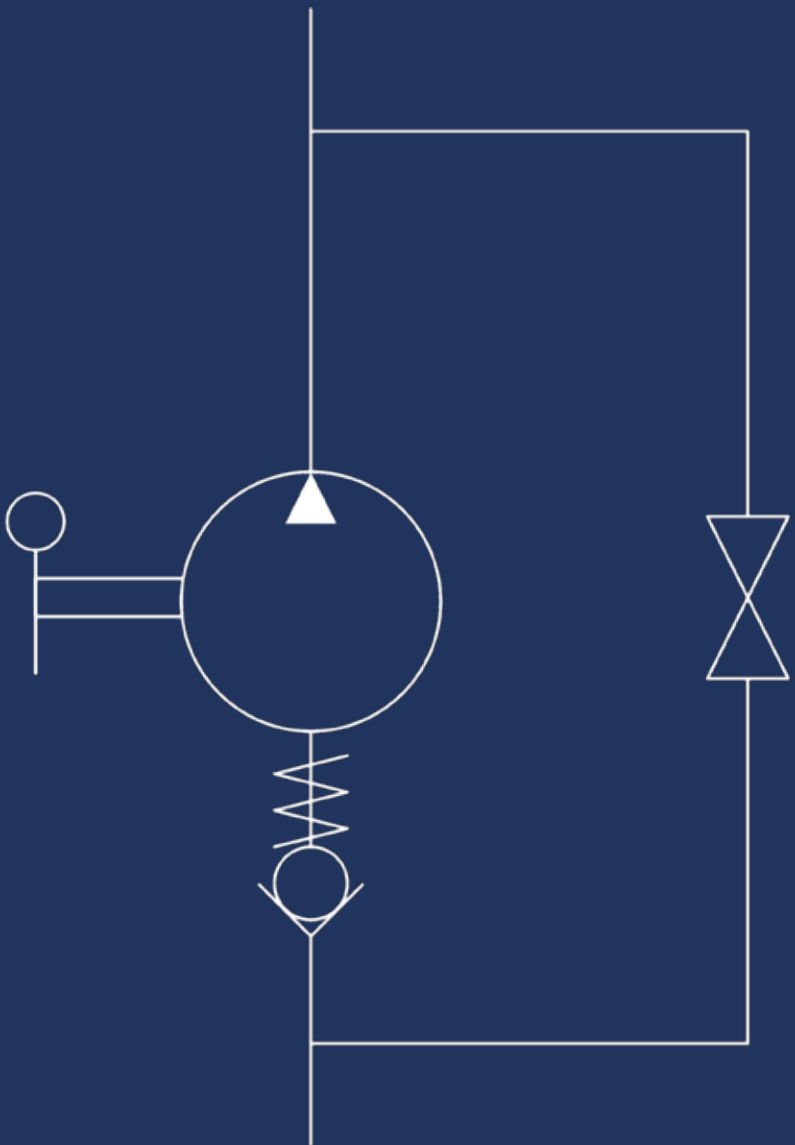
HYDRAULIC DIAGRAM
