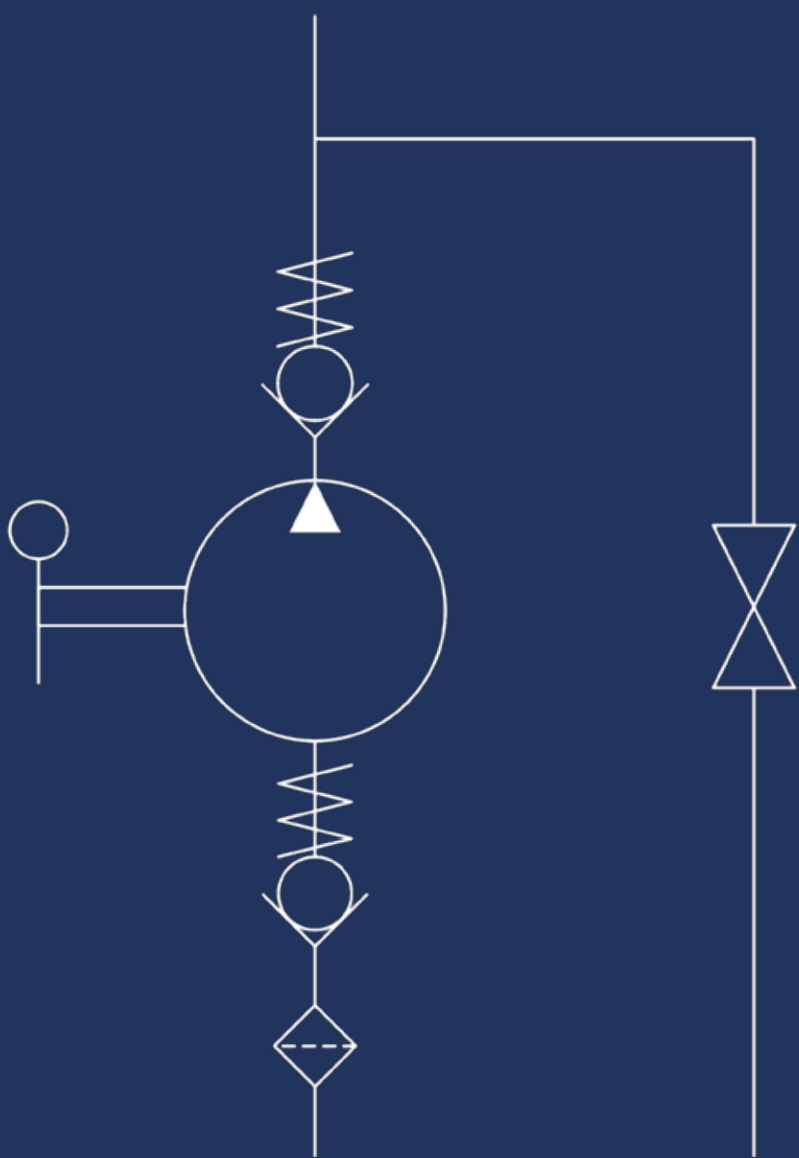
HYDRAULIC DIAGRAM
