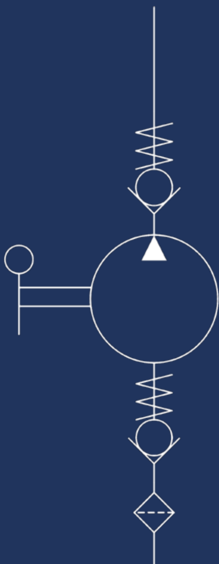
HYDRAULIC DIAGRAM
