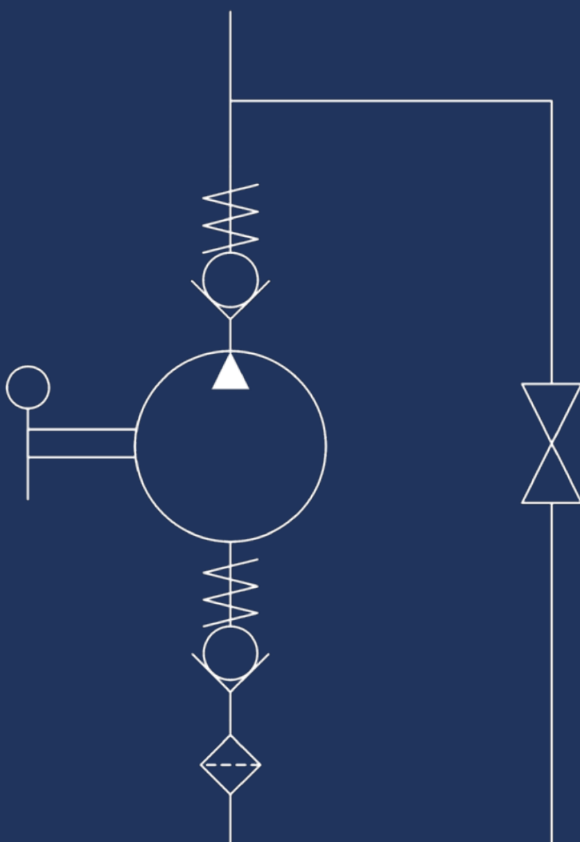
HYDRAULIC DIAGRAM
