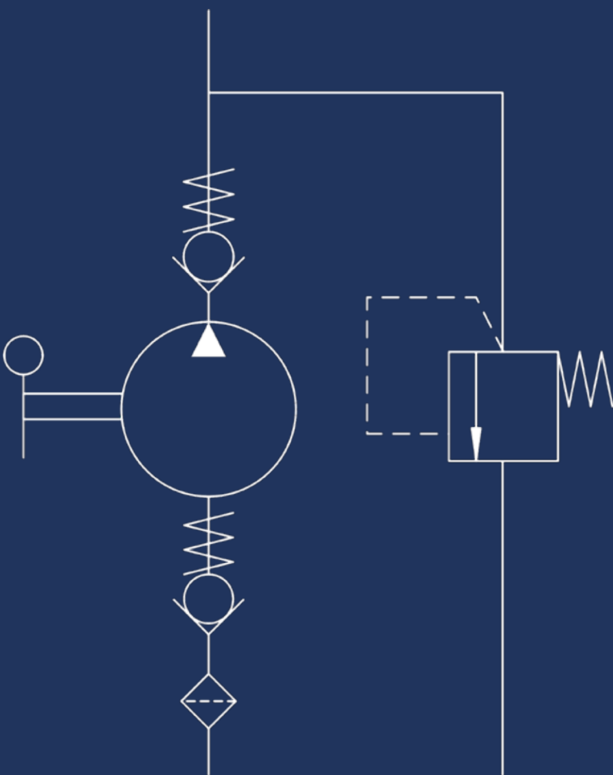
HYDRAULIC DIAGRAM
